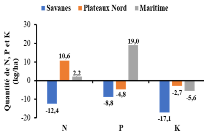
Figure 4: Average partial balance in N, P and K of cotton plots in the Savanes, Plateaux Nord and Maritime regions
