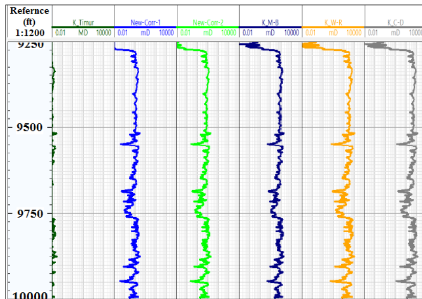
Figure 14: Estimated Permeability of Well A21-103
