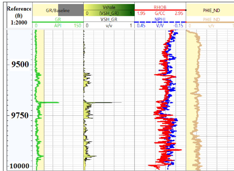
Figure 4: Porosity Estimation of well A11-103A
