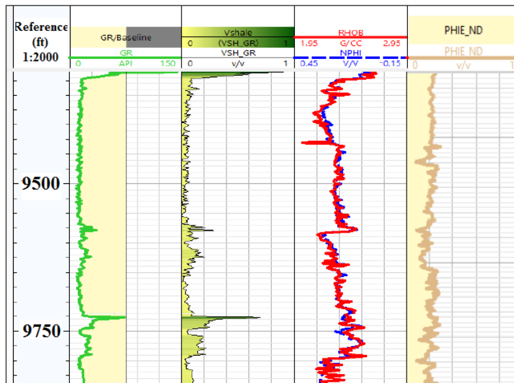
Figure 5: Porosity Estimation of well A16-103A
