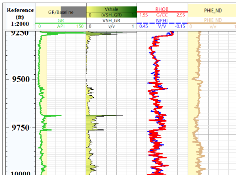
Figure 6: Porosity Estimation of well A21-103A
