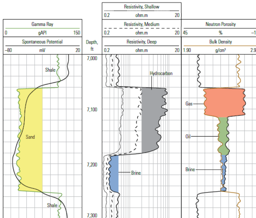
Figure 2: Quick look interpretation from Schlumberger company
