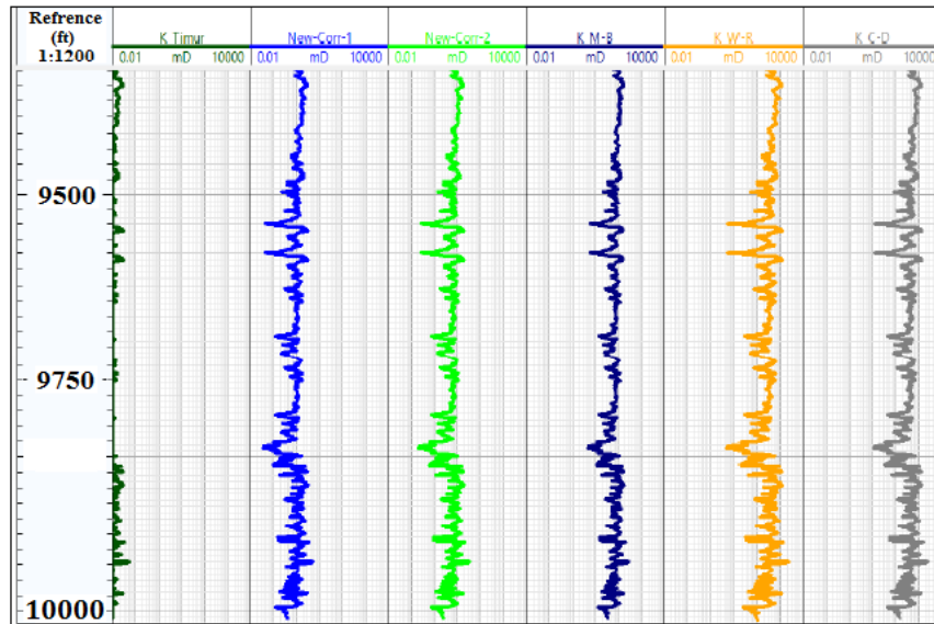
Figure 13: Estimated Permeability of Well A16-103A
