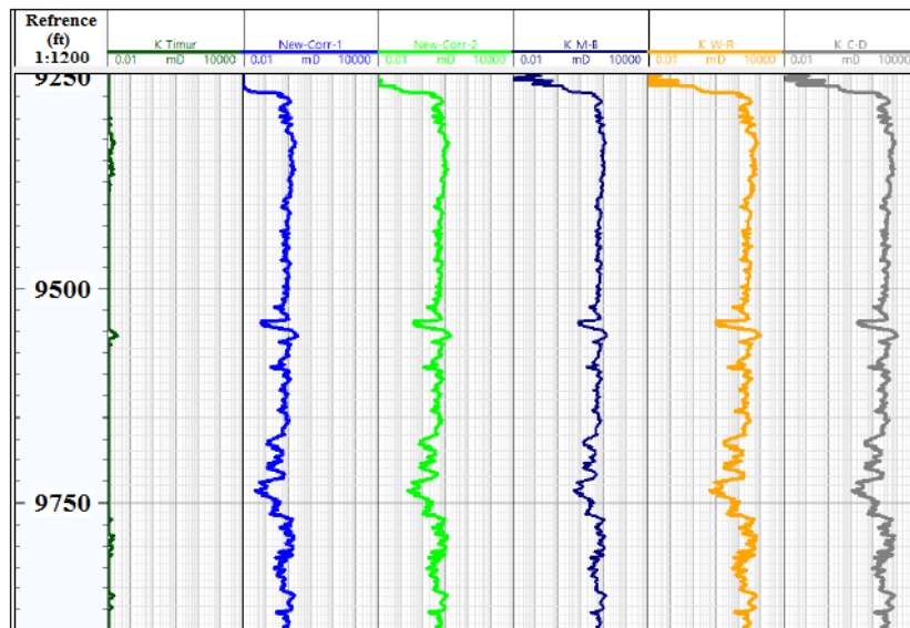
Figure 12: Estimated Permeability of Well A11-103A
