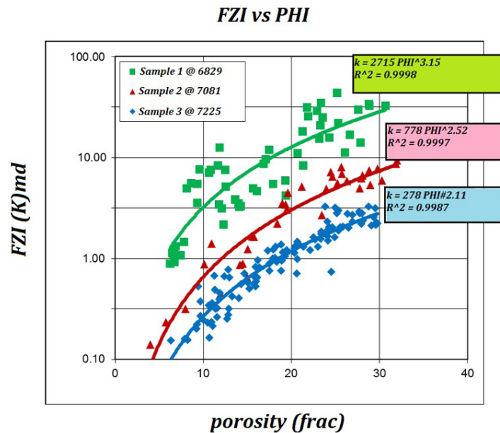
Figure 1: The relations between permeability and porosity for each HFU
