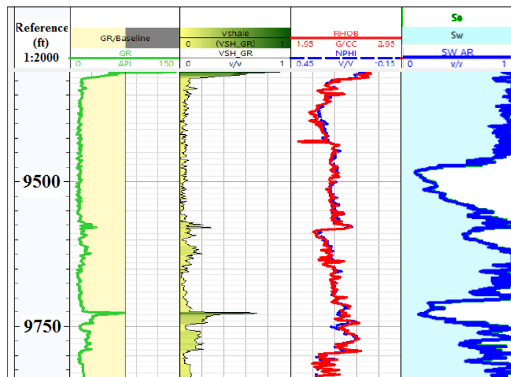
Figure 9: Water saturation of well A16-103A
