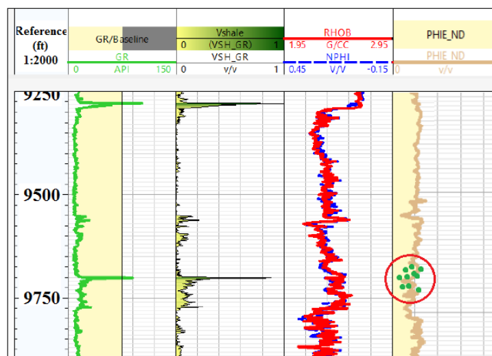
Figure 3: Porosity Estimation of well A7-103A
