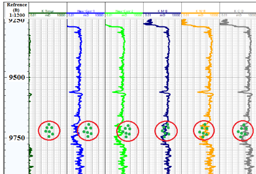
Figure 11: Estimated Permeability of Well A7-103A
