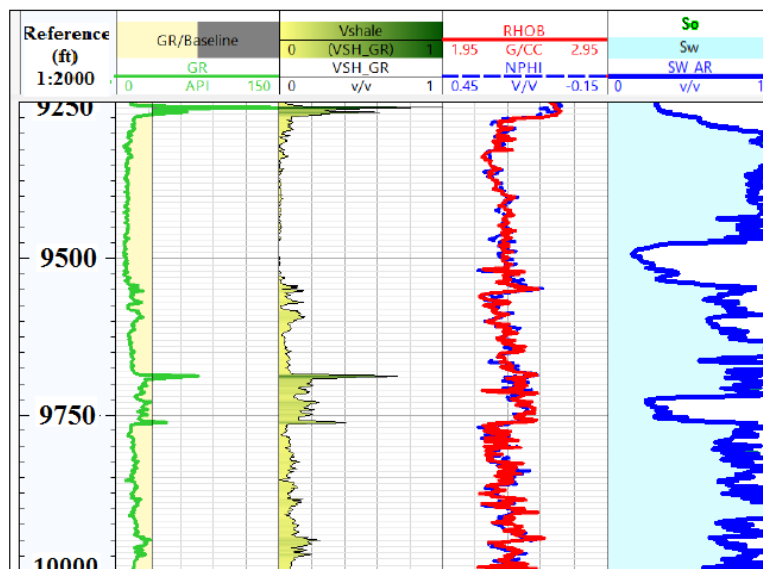
Figure 10: Water saturation of well A21-103A
