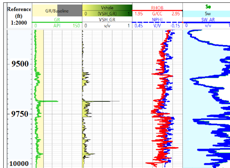
Figure 8: Water saturation of well A11-103A
