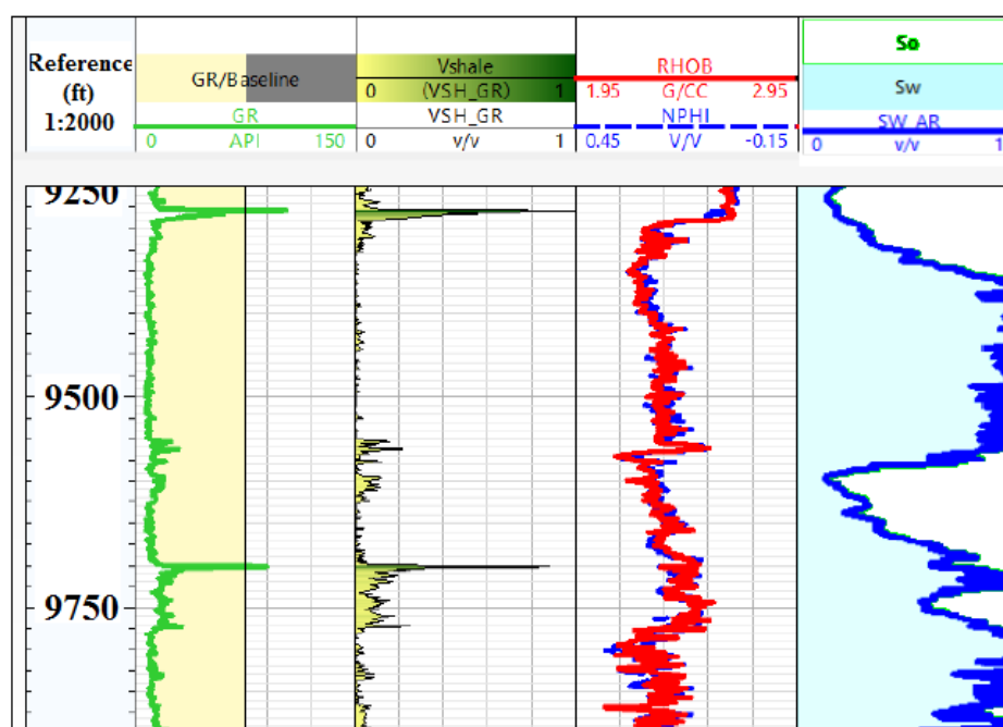
Figure 7: Water saturation of well A7-103A
