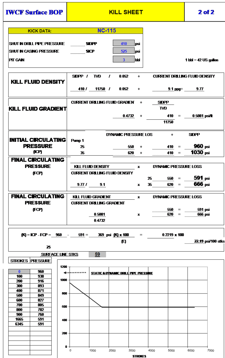
Figure 2: IWCF Surface BOF (Kill Sheet)
