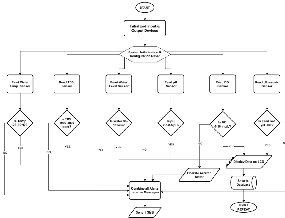
Figure 3: Hardware Flowchart
