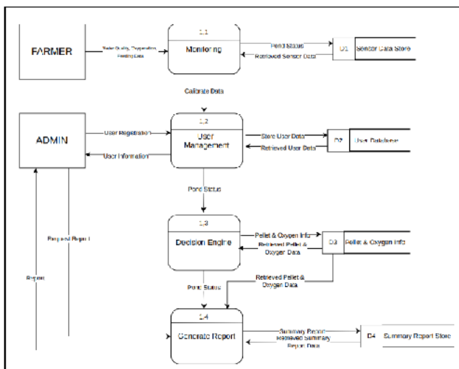
Figure 2: Data Flow Diagram (DFD) level 1
